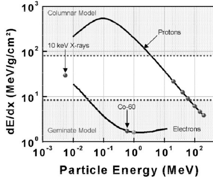
Comparison of Charge Yield in MOS Devices for Different Radiation Sources P.Paillet et. al.
