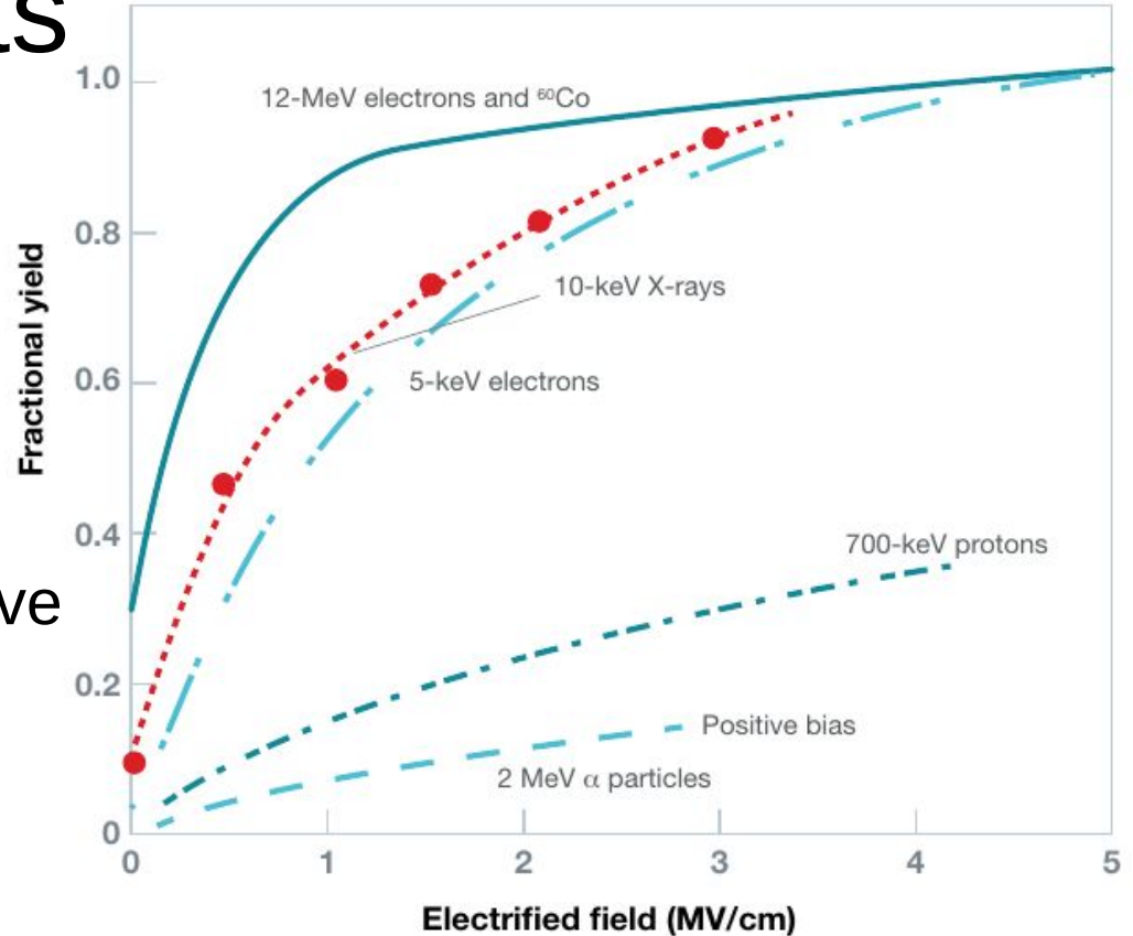
Figure 3-3. This diagram shows charge-yield fraction as a function of the oxide electric field for different types of ionizing radiation. [1] Note that more highly charged particles have a lower fractional yield.
