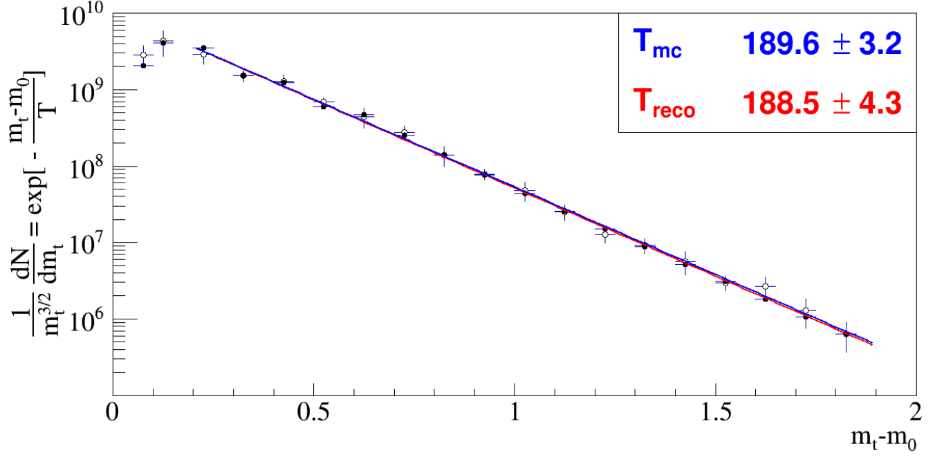
Figure 8.5: Amount of generated \pi^0 within the CBM acceptance obtained from MCtrue data bank (full circles) and from reconstructed pions after applying efficiency and acceptance corrections (empty circles). The blue and red lines show correspondingly a fit of full and empty circles using Formula 2.3.
