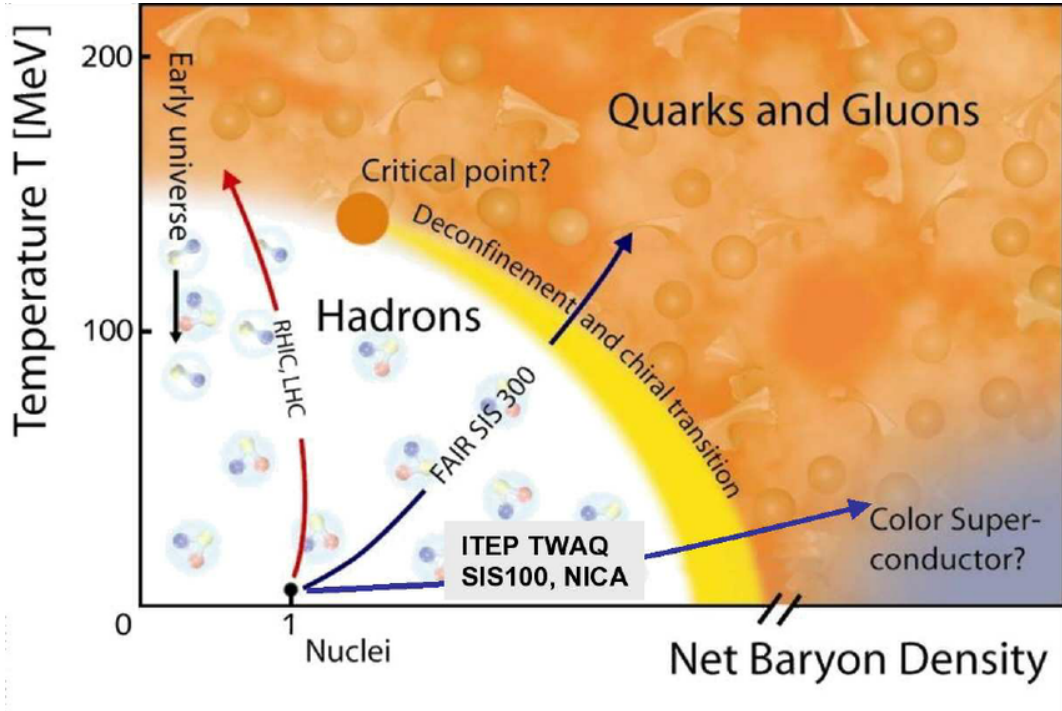
Figure 2.1: The illustration of possible phases of nuclear matter and their boundaries in a diagram of temperature T versus the net-baryon density \rho_B [10].
