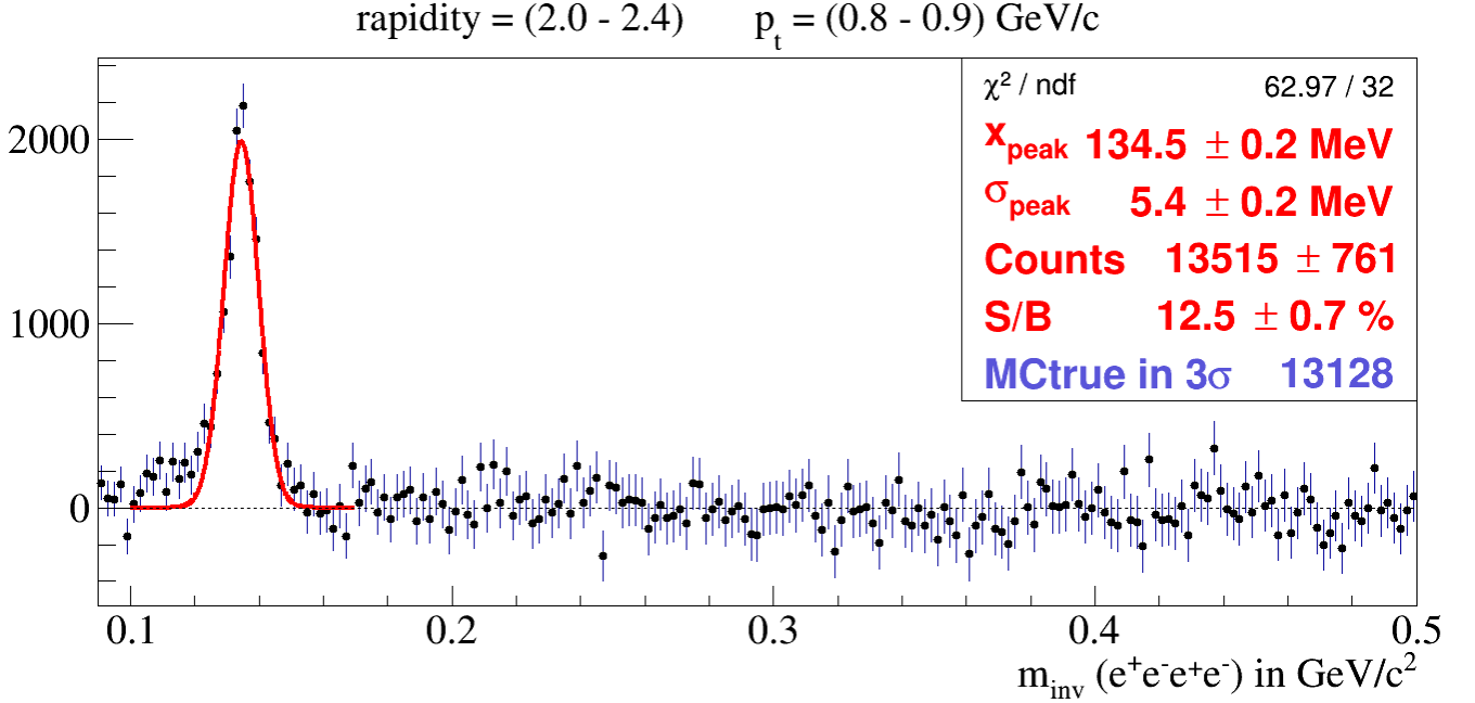
Figure 8.1: Background-subtracted \pi^0 invariant mass spectrum with cuts on photon candidates \Theta_{e^+e^-} < 2^\circ and m_{\text{inv}}(e^+e^-) < 20 \text{ MeV}/c^2 for a case with partial lepton identification within the RICH detector. The spectrum covers one particular phase space bin with rapidity y = 2.0 - 2.4 and transverse momentum p_t = 0.8 - 0.9 \text{ GeV}/c .
