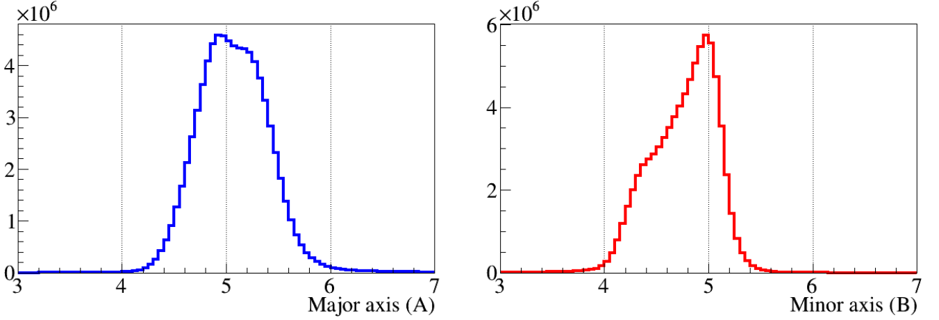
Figure 5.4: Major axis ( A ) and minor axis ( B ) distributions from the ellipse fit of projected ring images coming from electrons and positrons.
