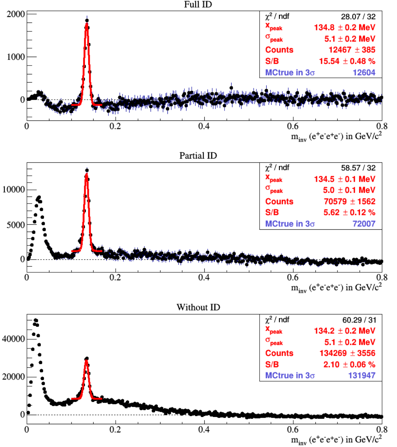
Figure 6.2: Two photon invariant mass spectra after background subtraction from the analysis with cuts m_{\text{inv}}(e^+e^-) < 20 \text{ MeV}/c^2 and \Theta_{e^+e^-} < 2^\circ using different lepton identification approaches: full (upper), partial (middle), without (bottom). Black dots show the background-subtracted spectrum and in red is shown the result of Gaussian fit to the peak region.
