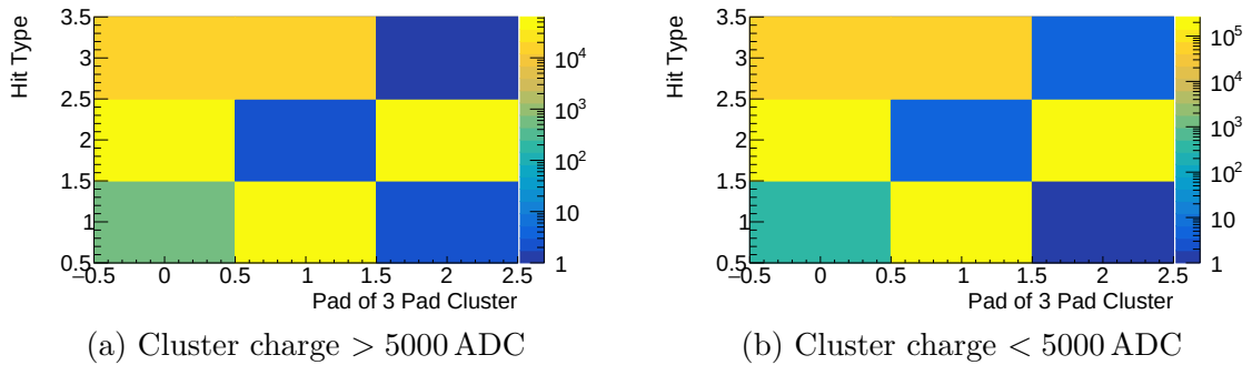
Figure 4.4.: These plots outline the hit types of the pads of three pad clusters with an integrated cluster charge > 5000 ADC (a) or < 5000 ADC (b). On the x-axis 0 is the left pad, 1 the middle pad and 2 the right pad of a cluster.
