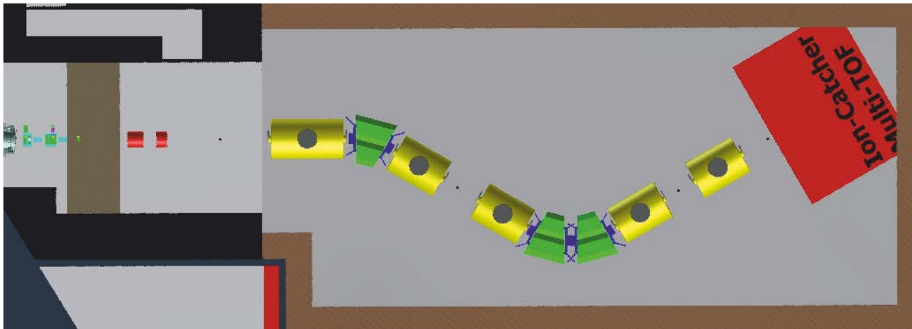
S-shaped energy buncher (dispersion matching to Super-FRS)
