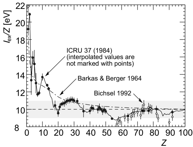
Figure 4.5: Average excitation energies divided by the atomic number as a function of Z . [104]
