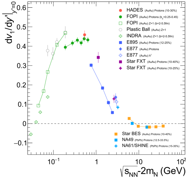
Figure 1.5: Excitation function of the directed flow slope (dv_1/dy)_{y=0} for protons as a function of the subtracted centre-of-mass energy \sqrt{s_{NN}} - 2m_N , compiled from various heavy-ion experiments.[24]
