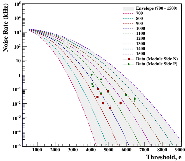
Figure 3.15: Noise rate as a function of discriminator threshold compared with Rice level-crossing predictions for different equivalent noise charge (ENC) values. The data points correspond to measured noise rates from run 2984.
