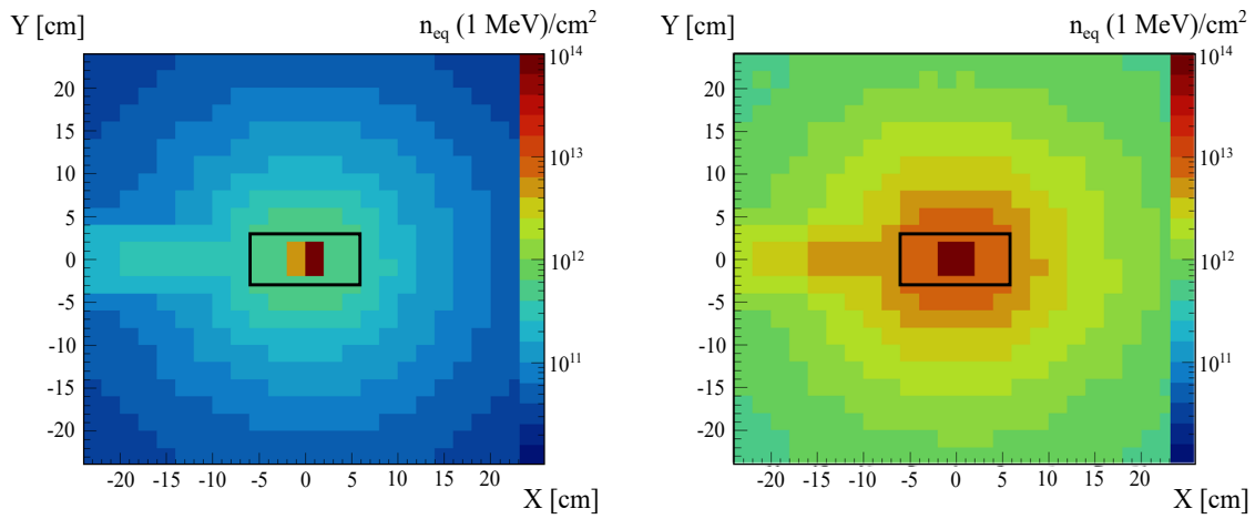
Figure 1.18: Fluence distribution of the first STS station located 30 cm away from the target. The simulation was performed using FLUKA, considering the 3-year running scenario with the highest beam intensity.[57, 58]
