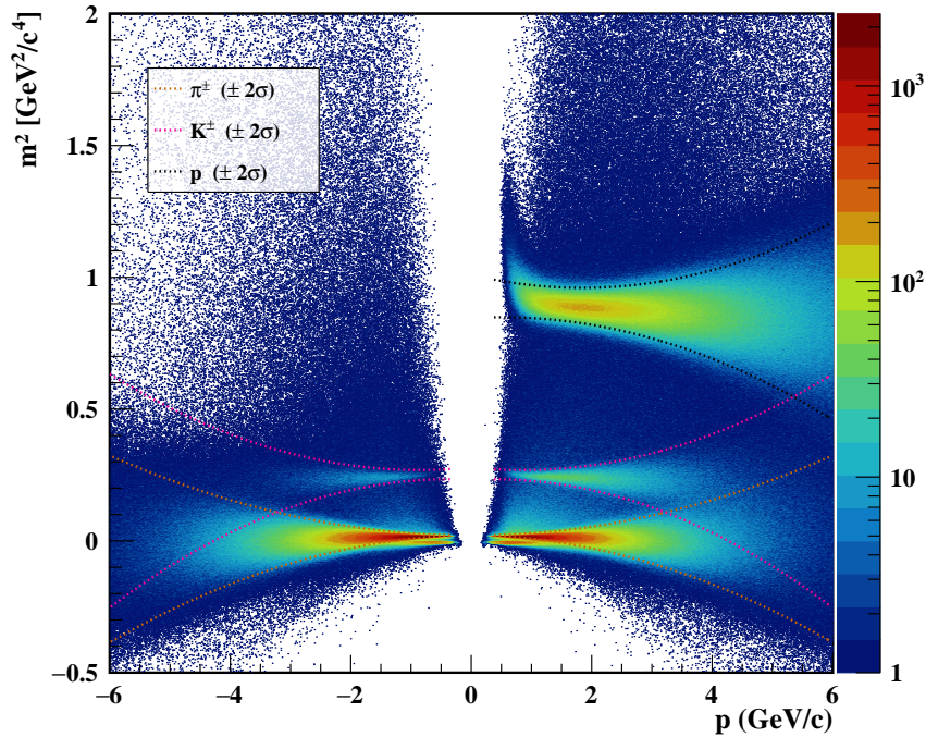
Figure 5.23: Mass-squared ( m^2 ) distribution as a function of momentum, calculated from the time-of-flight and track length. Bands corresponding to pions, kaons, and protons are visible and match the expected positions. The dotted curves represent \pm 2\sigma fit selection windows for each particle species.
