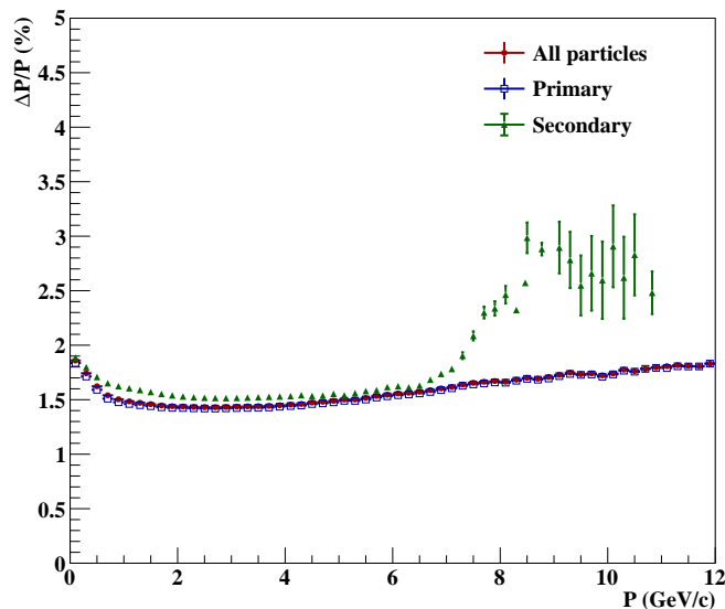
Figure 2.25: Momentum resolution \frac{\Delta p}{p}\% as a function of momentum for all charged, primary and secondary particles reconstructed in the STS, for an event generated for Au+Au collision at a beam momentum of 12 AGeV/ c and transported through the detector setup using CBM-ROOT.
