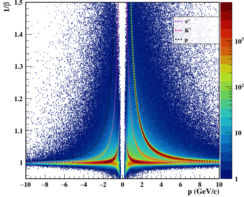
Figure 5.24: Inverse velocity ( 1/\beta ) as a function of momentum reconstructed from ToF measurements. The dashed curves indicate the expected positions of \pi^\pm , K^\pm , and p/\bar{p} . Distinct bands are observed, which converge at higher momenta where \beta \rightarrow 1 , reducing the separation power.
