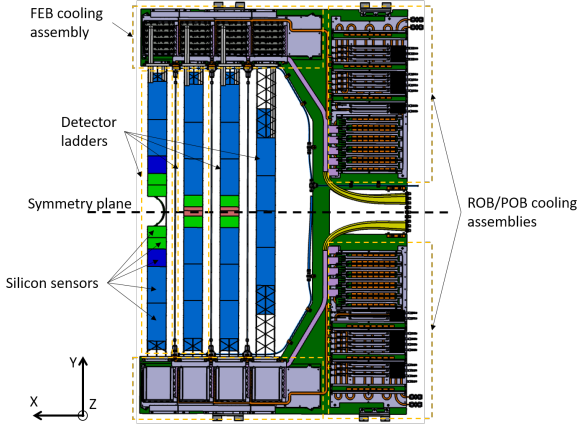
Figure 1.17: CAD model of the C-frame support structure for the ladders and other electronics components.
