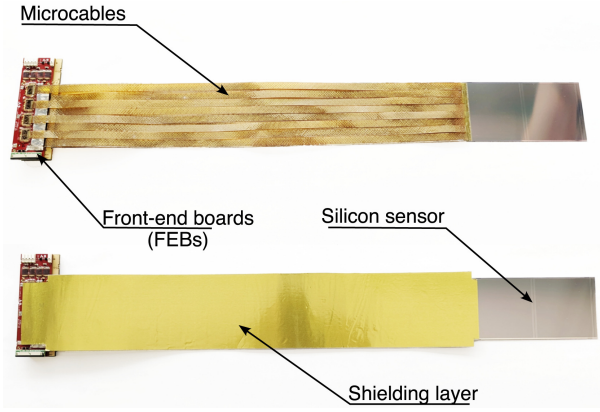
Figure 1.15: Sensors with micro-cables and Front-end-Electronics Boards known as Module.
