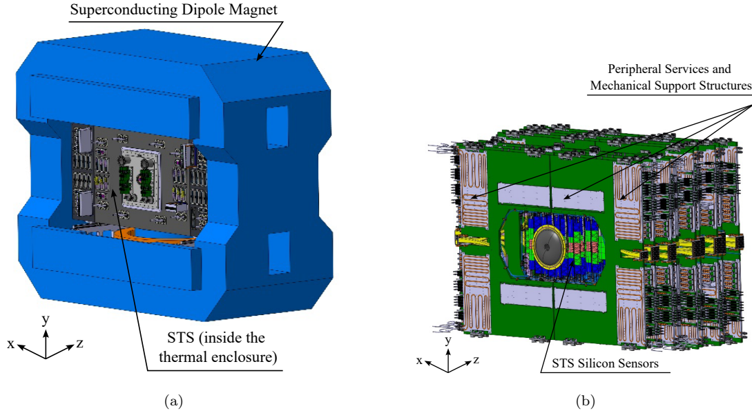
Figure 1.13: Figure 1.13a shows a CAD model of the STS detector system placed inside the magnet, and Figure 1.13b represents the active area and peripheral mechanical support structure.
