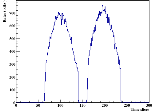
Figure 3.4: BMON detector spill rates
