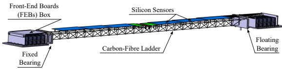
Figure 1.16: CAD model of the CF-ladder along with a sensor mounted on it and other electronics components.
