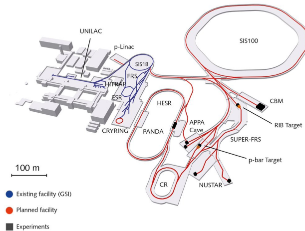
Figure 1.11: Layout of existing and planned GSI-FAIR facility along with the various experimental sites marked in black dots.
