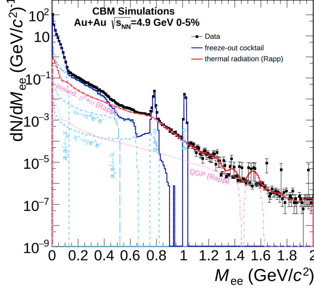
Figure 1.8: Invariant mass spectrum of e^+e^- pairs radiated from a central Au+Au collision at 4.9 GeV.[33]
