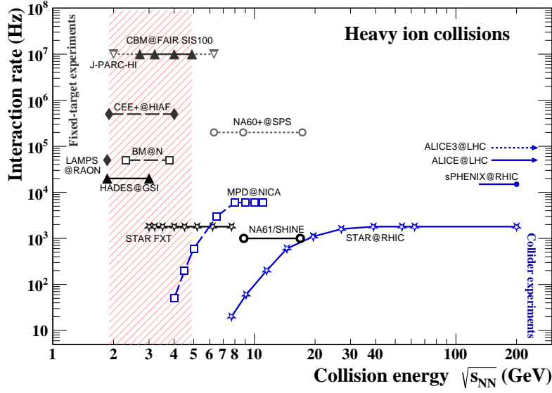
Figure 1.4: Interaction rate of the different heavy-ion physics experiments as a function of collision energy ( \sqrt{s_{NN}} ). Various fixed-target and collider-based heavy-ion physics facilities, existing, planned, and under construction, are marked in black and blue colors, respectively, adapted and modified from [21].
