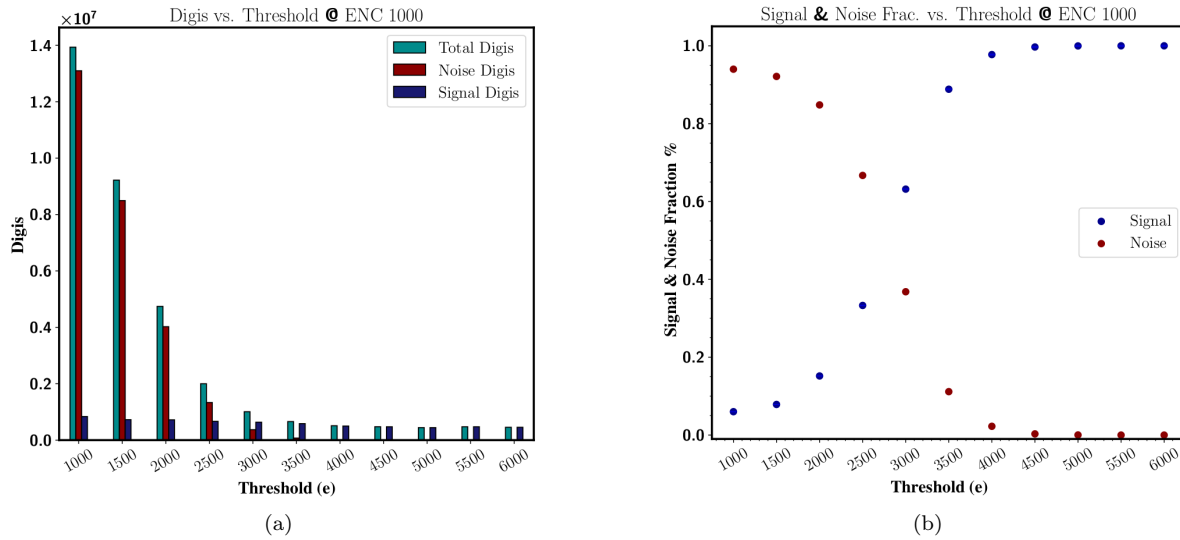
Figure 4.14: Figure 4.14a shows total, noise, and signal digs distribution at ENC 1000 e while Figure 4.14b represents Signal to Noise fraction at varying threshold values.
