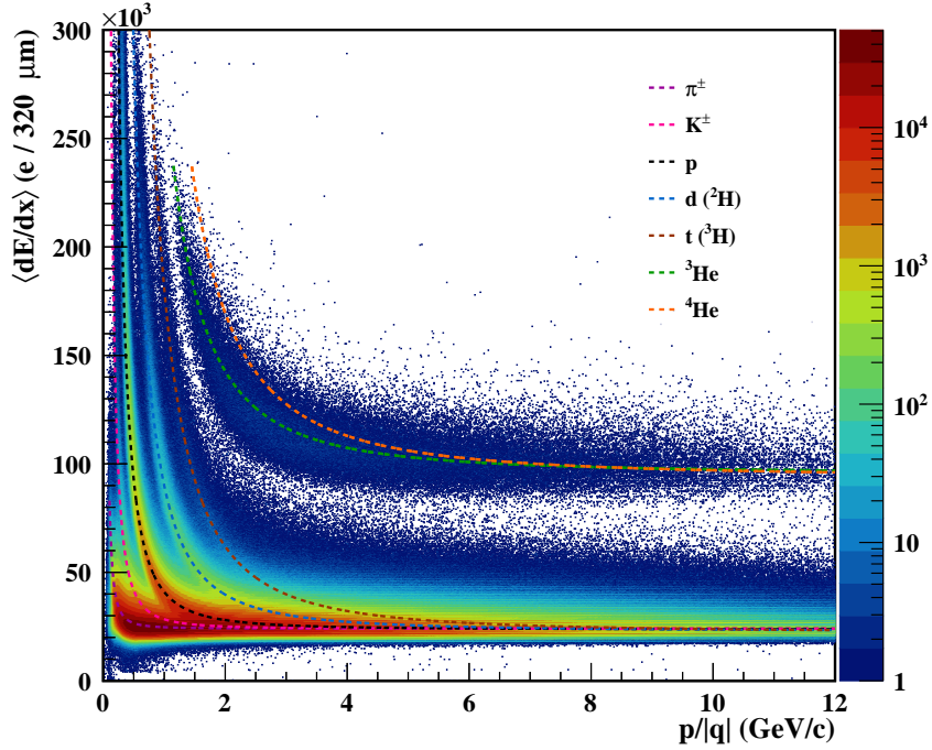
Figure 5.25: Specific energy loss \langle dE/dx \rangle (normalized to 320 \mu\text{m} ) as a function of momentum-to-charge ratio p/|q| , reconstructed with the STS from PHQMD-simulated Au+Au collisions at beam momentum 12 AGeV/c. The dashed curves indicate the expected Bethe-Bloch dependence for different particle species.
