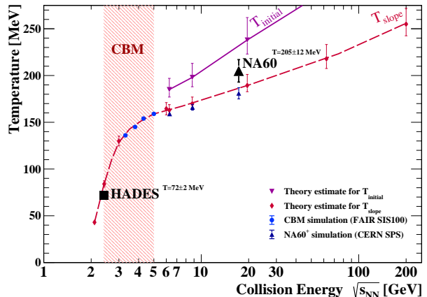
Figure 1.9: Compilation of measured and estimated effective fireball temperatures as a function of the Center-of-Mass (COM) energy per nucleon pair, \sqrt{s_{NN}} . The black markers represent experimental results from HADES and NA60, respectively, corresponding to the extracted slope and initial temperatures of the medium. The red dashed curve indicates a theoretical interpolation of the thermal evolution, while the blue circles mark the projected sensitivity and energy coverage of future measurements with the CBM experiment at FAIR.[38]
