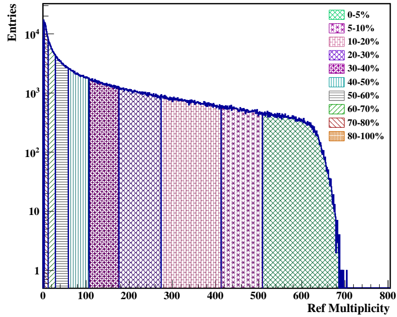
Figure E.1: Multiplicity distribution of charged particles for UrQMD model-based generated events of Au+Au interaction at 12 AGeV/c and classified into different centrality classes.
