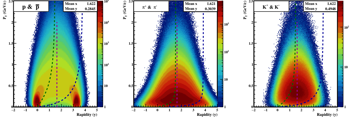
Figure 5.2: 4\pi distribution of transverse momentum ( p_T ) vs. rapidity ( y ) for protons, antiprotons, charged pions, and charged kaons from UrQMD minimum-bias events from Au+Au collisions at beam momentum 12 AGeV/c. The line at mean X in each panel shows the mid-rapidity. The green and blue lines represent the kinematic cuts of detector acceptance, 1.5 \leq \eta \leq 3.82 , representing polar angle 2.5^\circ < \theta < 25^\circ . The full 4\pi distribution is shown here for reference.
