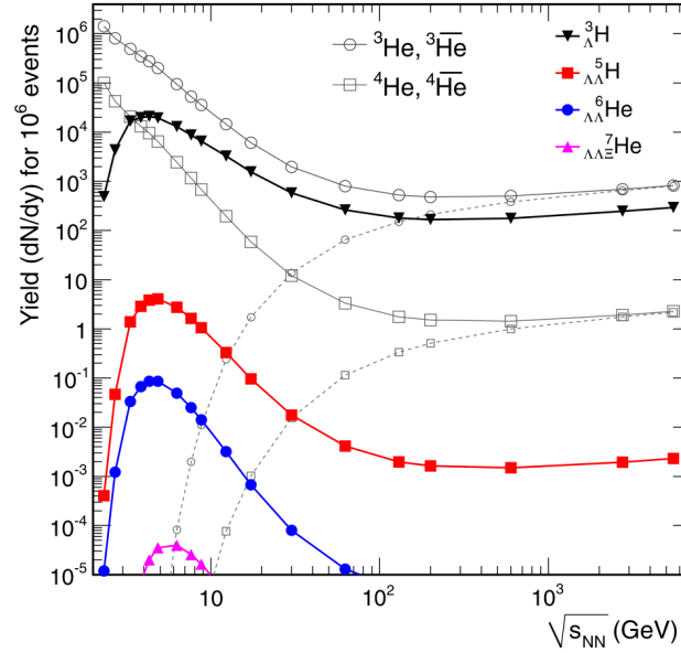
Figure 1.10: Predicted yield of hypernuclei at mid-rapidity vs. energy.[50]
