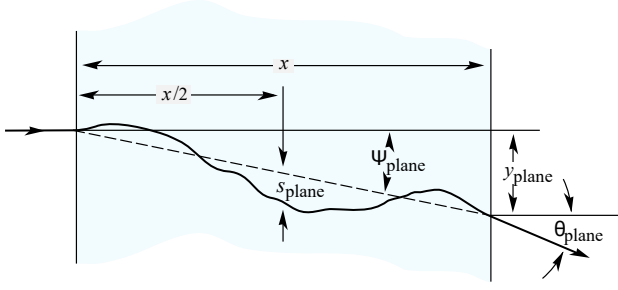
Figure 2.1: Illustration of dispersion of incident particle by \theta_{plane} due to multiple Coulomb scattering while passing through the detector layer of the thickness x . [46]
