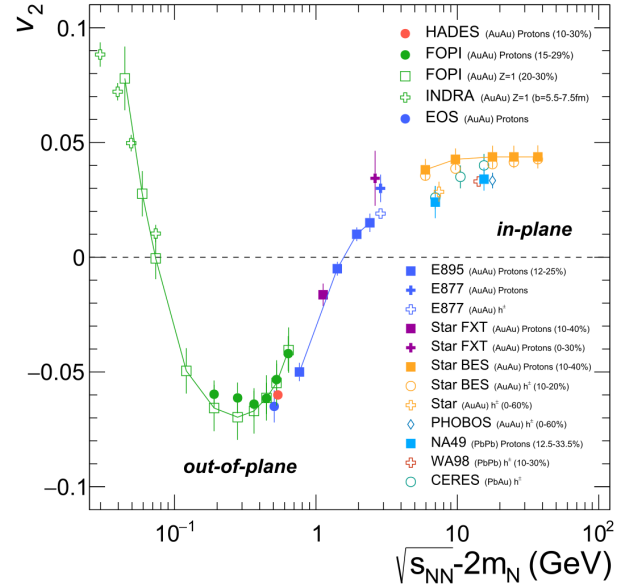
Figure 1.6: Excitation function of the elliptic flow coefficient v_2 for protons and light charged particles from different experiments.[24]
