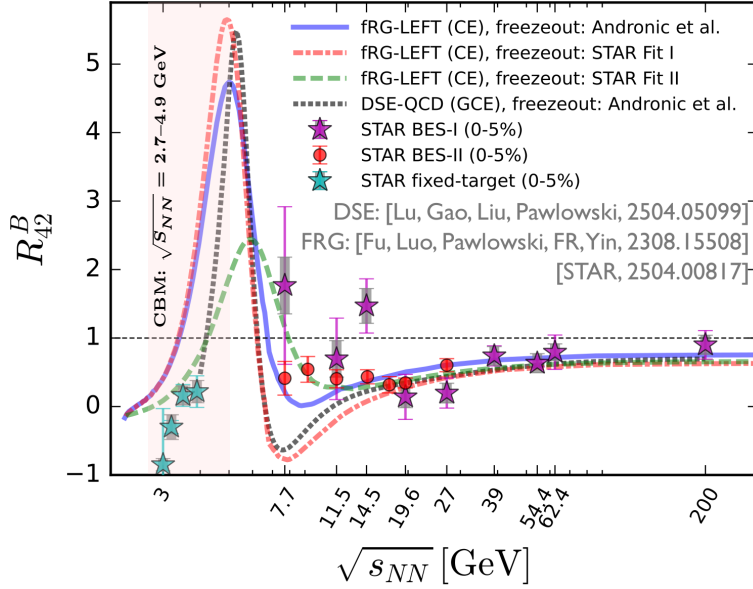
Figure 1.7: Energy dependence of the baryon number fluctuation from various theoretical model-based predictions and net-proton fluctuation data points for kurtosis \kappa\sigma^2 in most-central Au+Au collisions measured at the STAR experiment (RHIC) [28, 29]. The shaded band indicates the CBM@FAIR energy window.[31]
