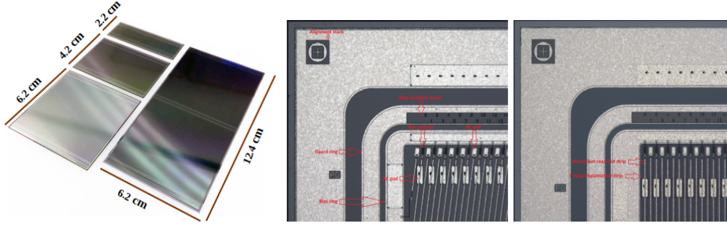
Figure 1.14: Double-sided double metal microstrip silicon sensor of four different variants used in the eight tracking stations of the STS detector
