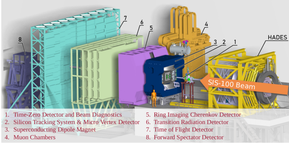
Figure 1.12: CBM experiment detector setup.
