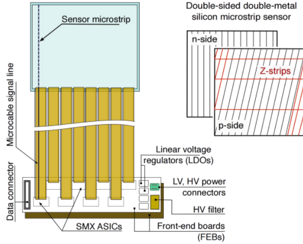
Figure 4.2: Schematic of the silicon sensors and their connection with the micro-cables and the ASICs.[100]
