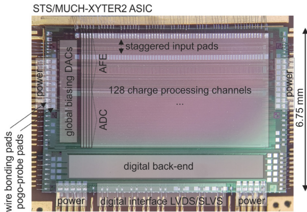
Figure 4.1: Layout of so-called STS-MUCH XYTER ASICs.[99]
