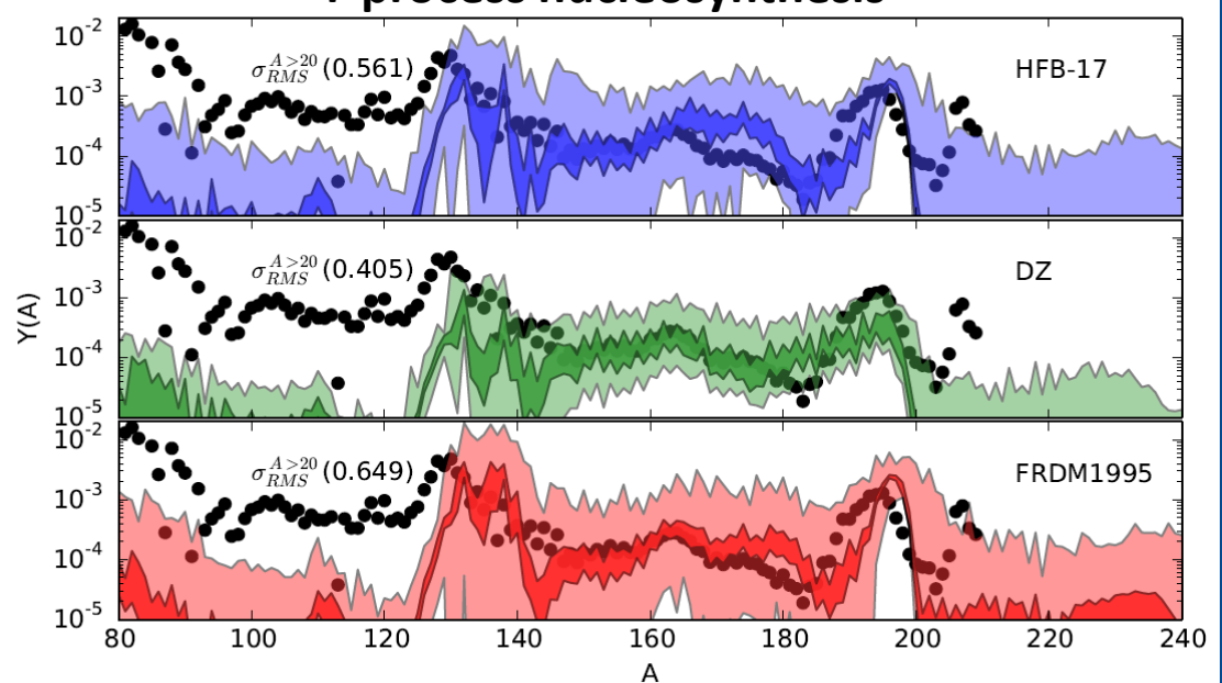
r-process nucleosynthesis
