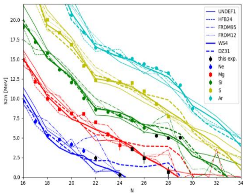
Nuclear mass data
