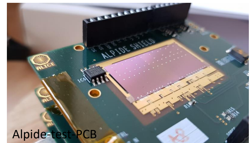
wirebonding with 25 µm Aluminum wire
