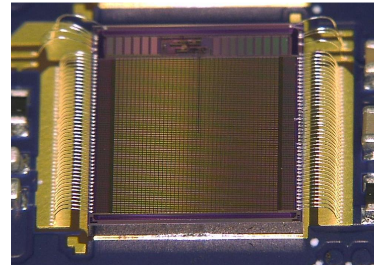
wirebonding with 25 µm Aluminum wire
