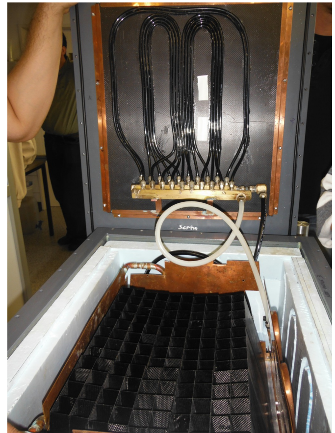
Final PROTO120 casing
