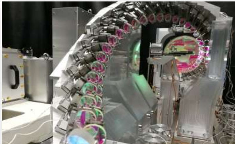
ELI-NP Gamma beam source laser-electron interaction chamber
