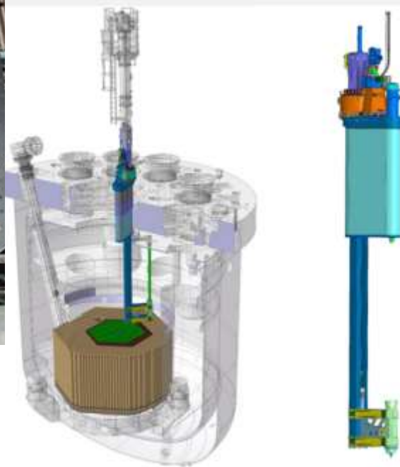
CEA Phenix Hot Cell Remote Handling
