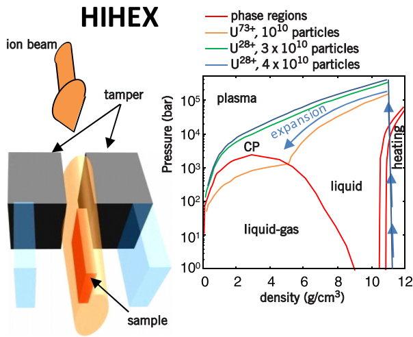
FIG. 3. The HIHEX scheme where ion beams ( U^{28+} or U^{73+} ) heat a material sample confined between two tampers. The sample heats isochorically with subsequent isentropic expansion. Using the SIS-100 parameters envisaged for FAIR Day-one experiments, the HIHEX scheme will be able to fully explore the critical points of many periodic system metals. Right-hand side: HIHEX predictions for lead for various ion-beam intensities. 54
