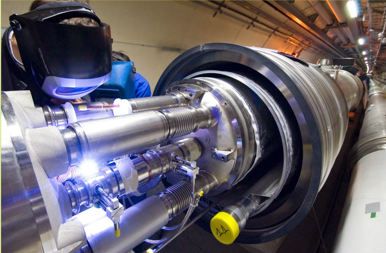
Demaco technicians are connecting the sections on site.
