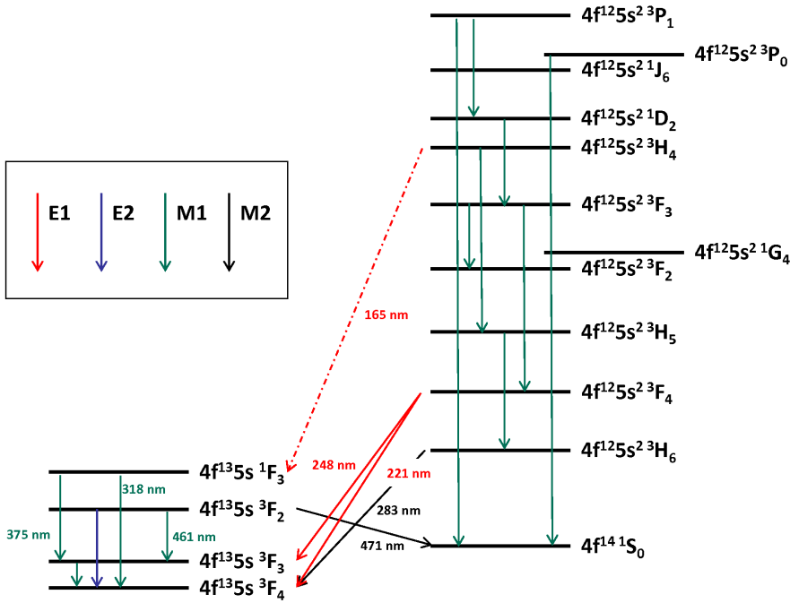
Fig. 2 Partial level scheme and transitions wavelengths in \text{Ir}^{17+} based on ref.[3]. Energy positions are not drawn to scale.
