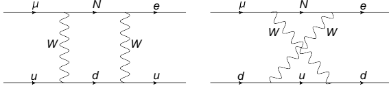
Fig. 4 Some box diagrams that contribute to the muon to electron conversion in presence of right-handed neutrinos.
