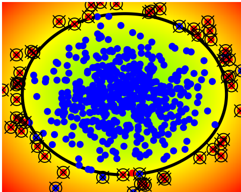
One Class SVM # N 500 # O 50
