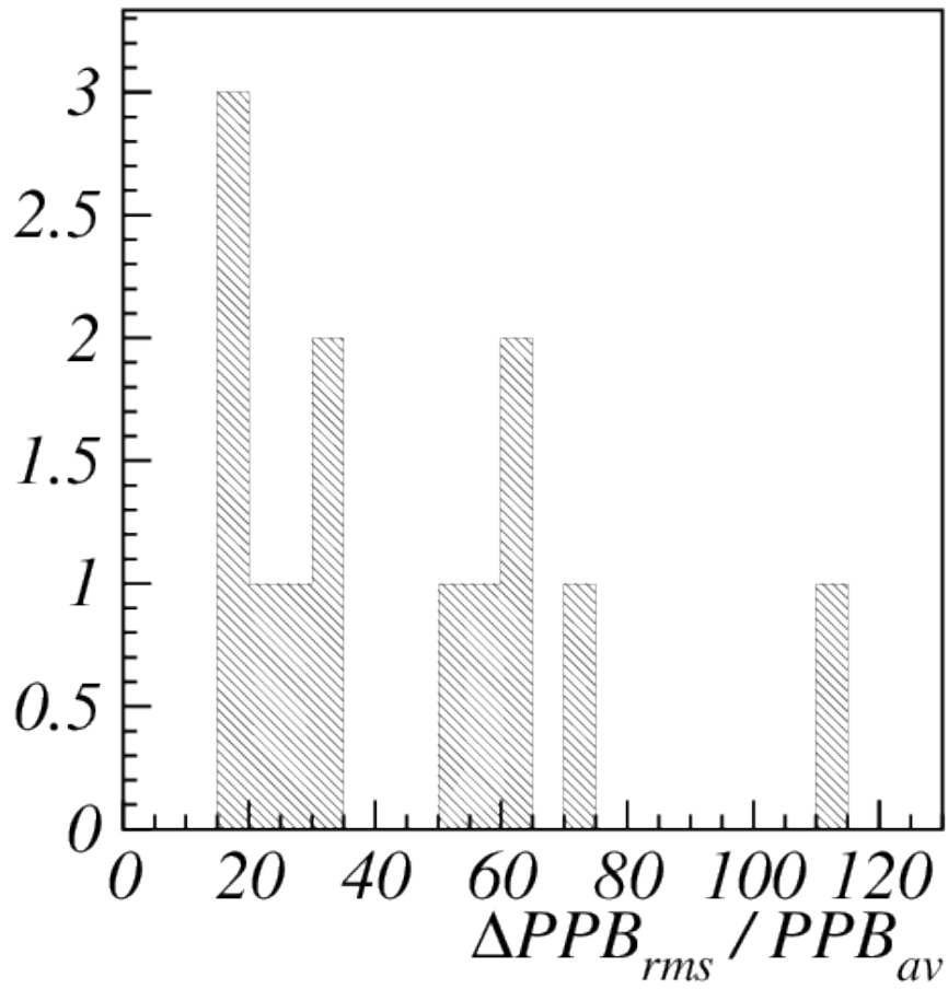
Fig. 2. Frequency of the “spill structure fluctuations”. The result is that no facility is able to produce a spill structure with relative fluctuation less than 15%. The majority of the spills are in the 15-35% range, and another group of spills is in the 50-80% range.
