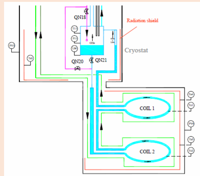
Cold mass of the cryostat
