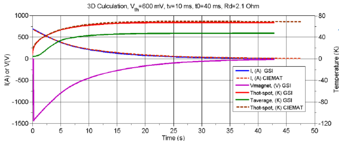
Figure 34. 3D quench calculation of the CBM dipole - magnet current, magnet voltage and the maximum (hot spot) coil temperature
